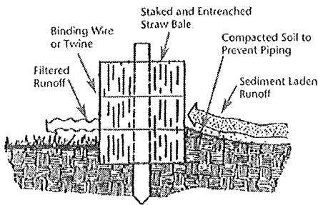
Cross Section of Straw Bale Installation
