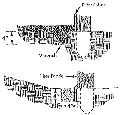
Cross Sections of Trenches for Silt Fences
